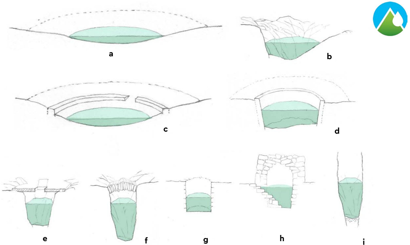
a) pond with shelving shores and no encircling wall, b) pond partially embedded between stone blocks of bedrock, c) pond with a shorter dry stone retaining wall, d) pond with a taller dry stone retaining wall, e) cistern embedded between stone blocks and covered with a concrete slab, f) cistern embedded between stone blocks and vaulted with stone, g) open well, h) corbel-vaulted well, i) karren well
